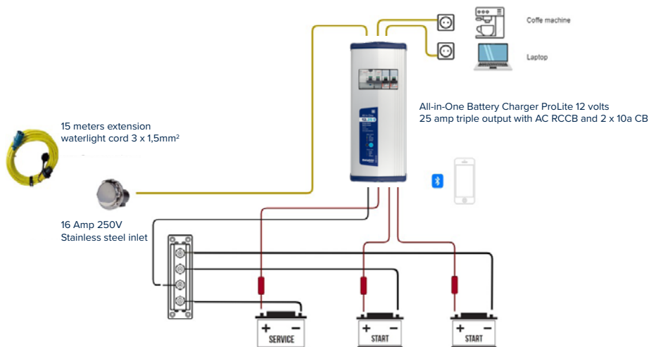
Triple battery bank system with All-in-One ProLite 12V25A battery charger and shore power kit
